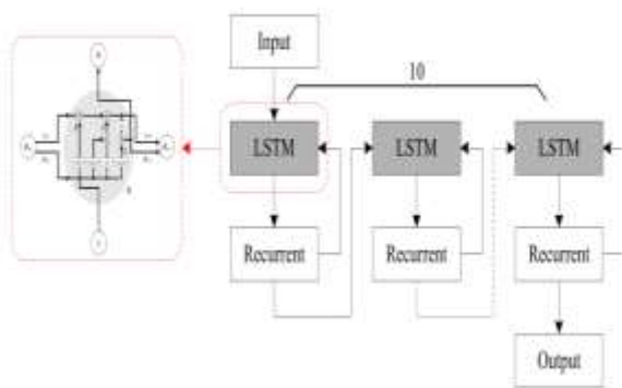
LSTM RNN architecture is shown in Fig. 4.
